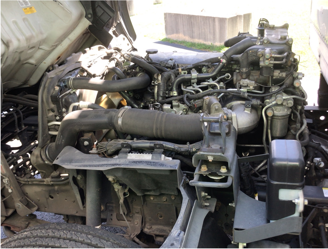
Engine Compartment / 08-31-2023
