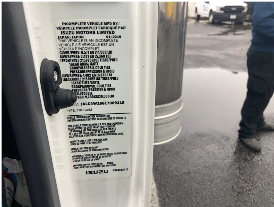
VIN: JALC4W166L7009318 / GVWR: 14,500 lbs / Axle Information / 12-15-2023
