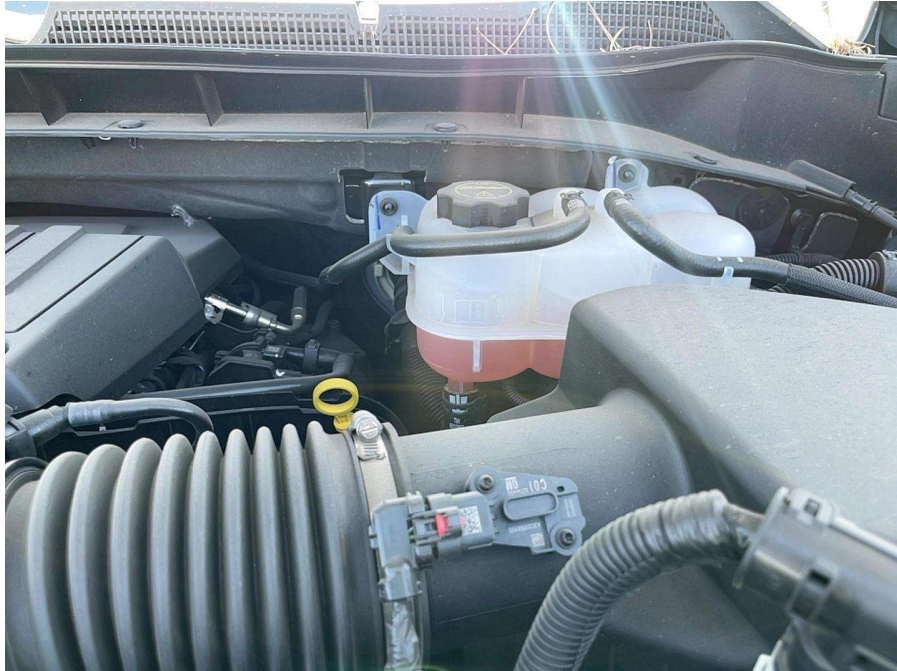
Coolant Level
