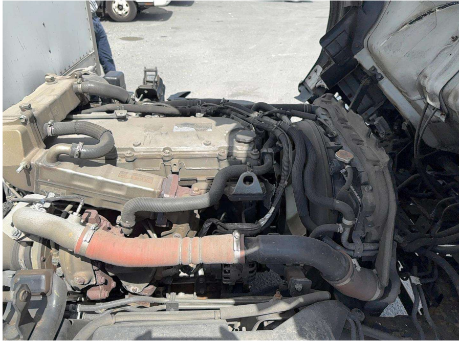
Engine Compartment
