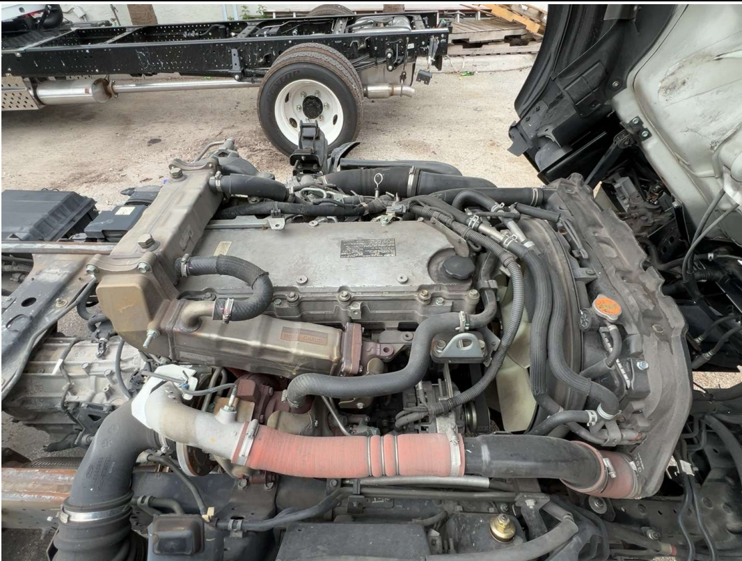
Engine Compartment / 11-29-2023
