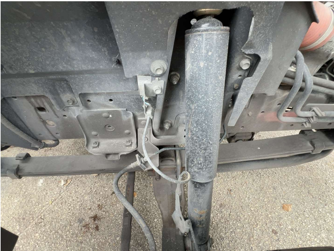
Axles / Suspension / 11-29-2023
