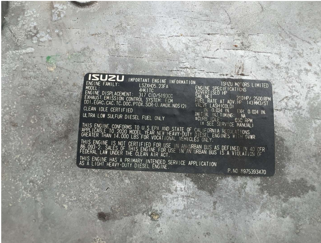
Engine Information / 11-29-2023
